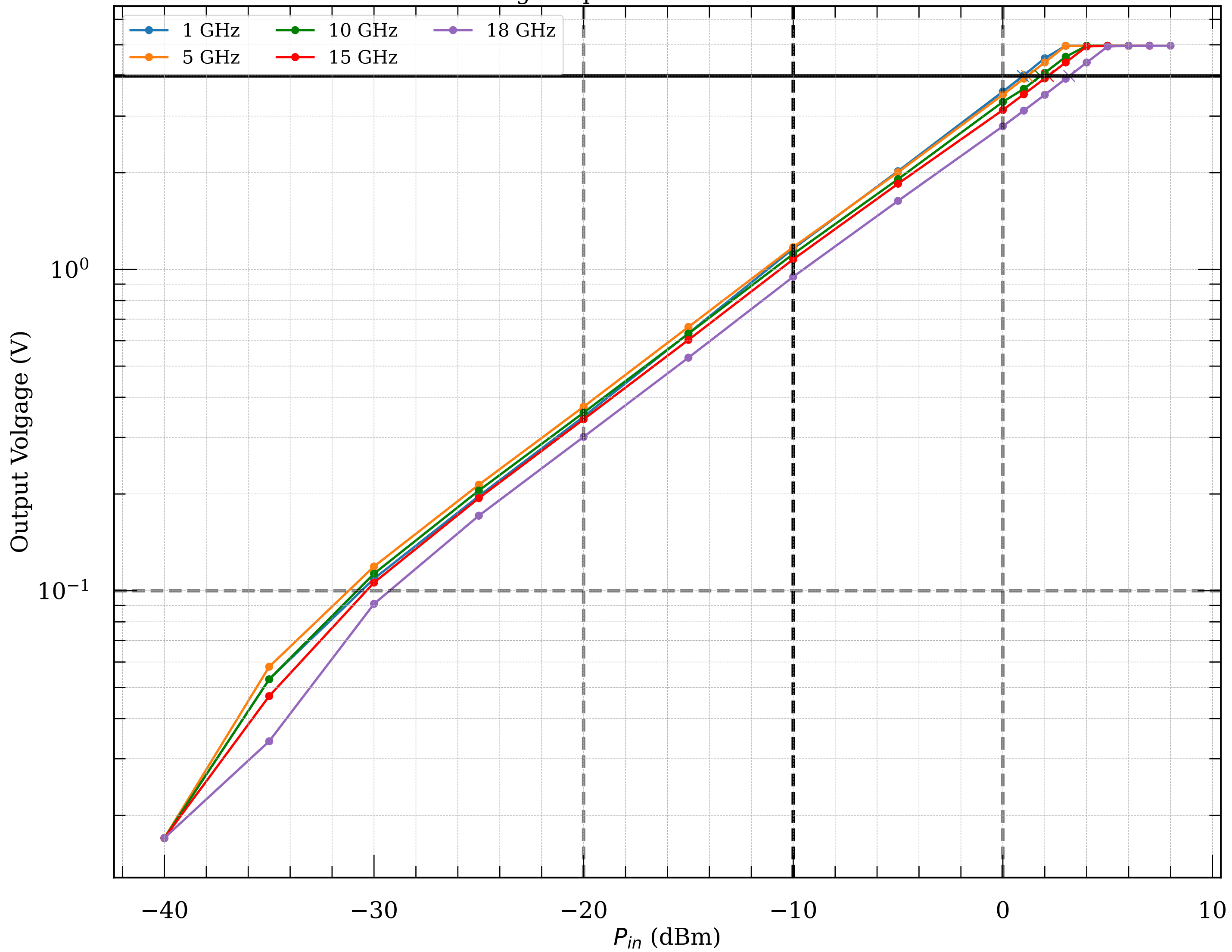
Measured voltage-to-power curve of detector module067
